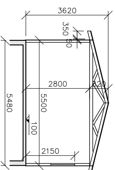
SNID 1:100
